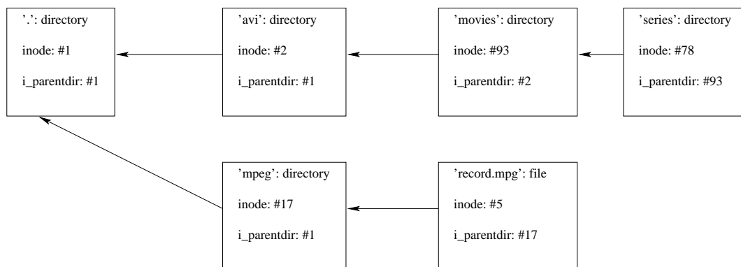
Figure 3.3: Nesting of directories
