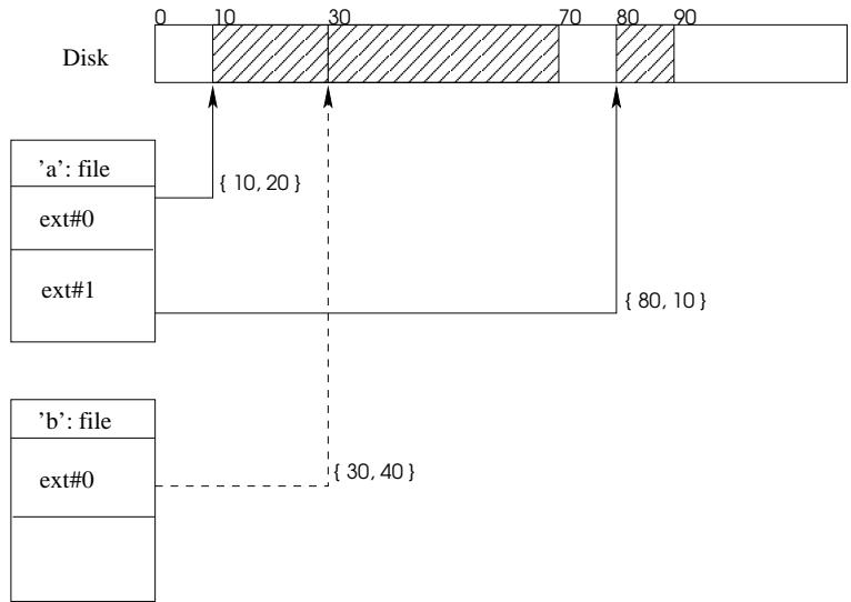
Figure 3.6: File-extent administration
